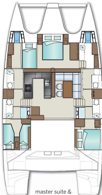
master suite & 3 guest cabins option
