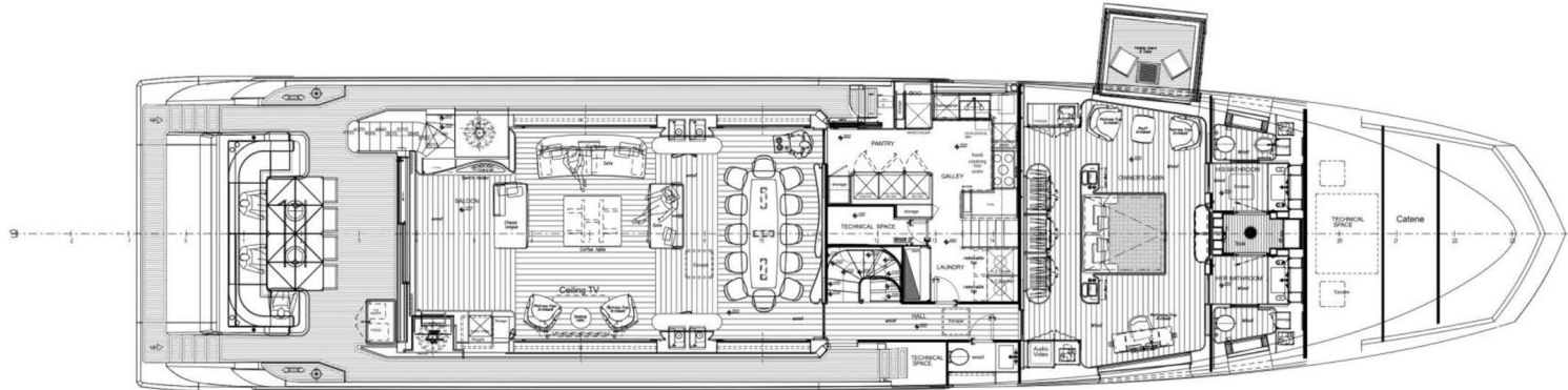
Main deck
